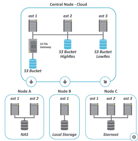
Evolution aSTORM Architecture
